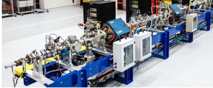
Neutron beams to explore the femtoscale (MONNET)
