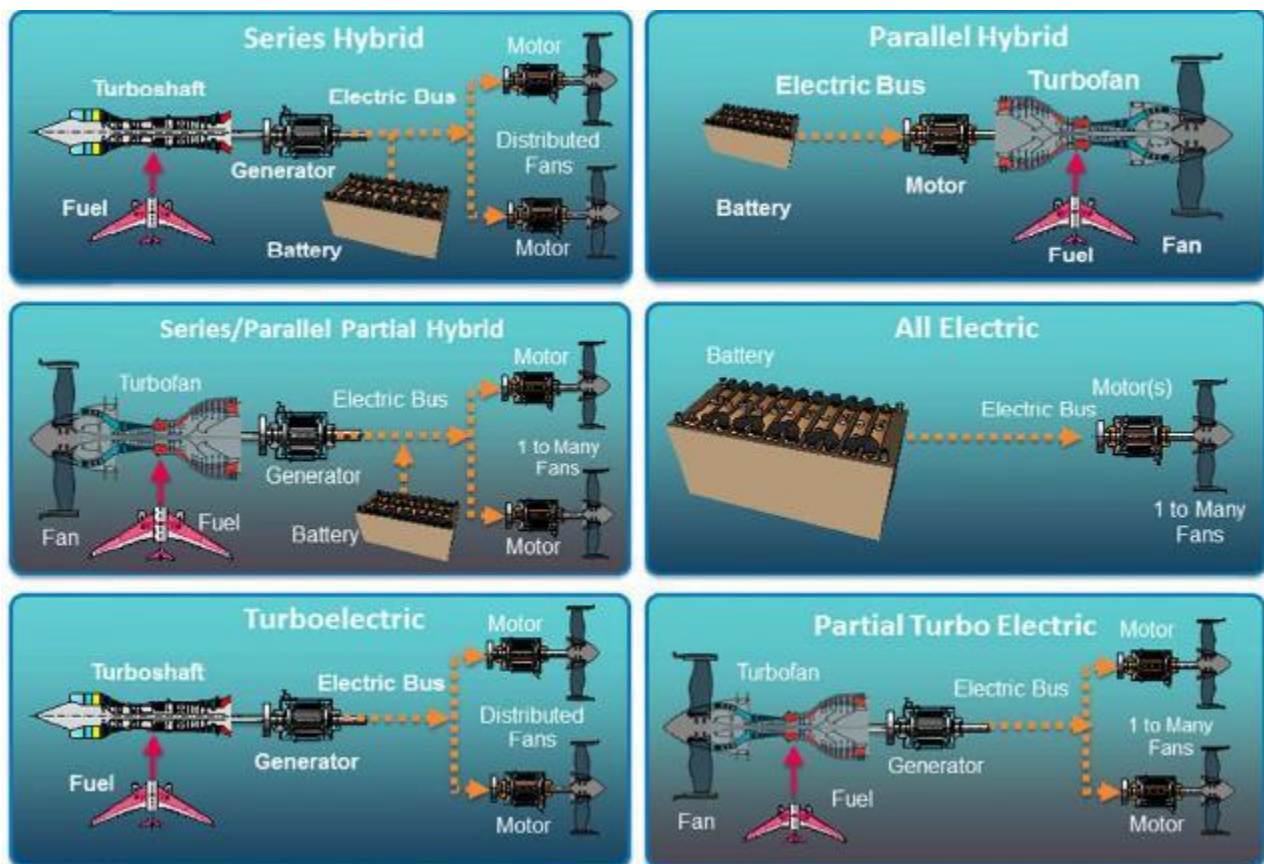
Figure 3.1: Electric Propulsion architectures
