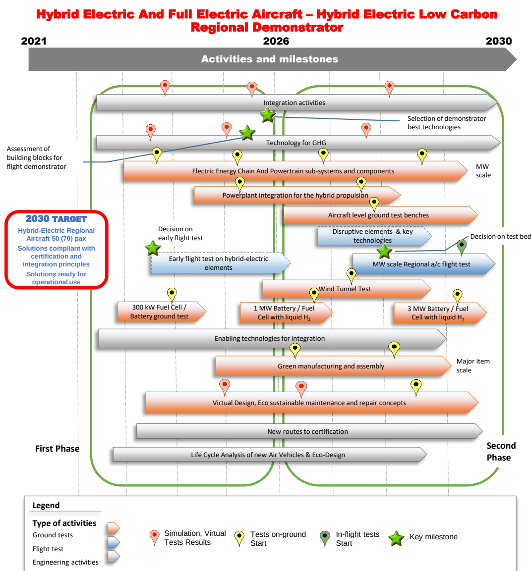
Figure 3.3: Regional Aircraft Integrated Planning
