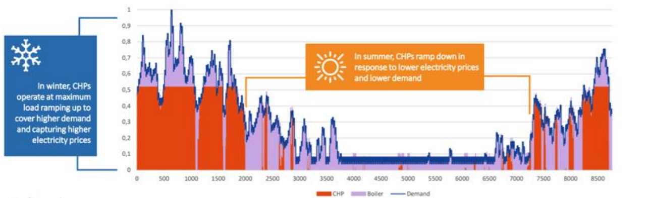
Figure 19. CHP Hourly operation - example for a thermosensitive heat demand (district heat for buildings) (source: Artelys, 2020)
