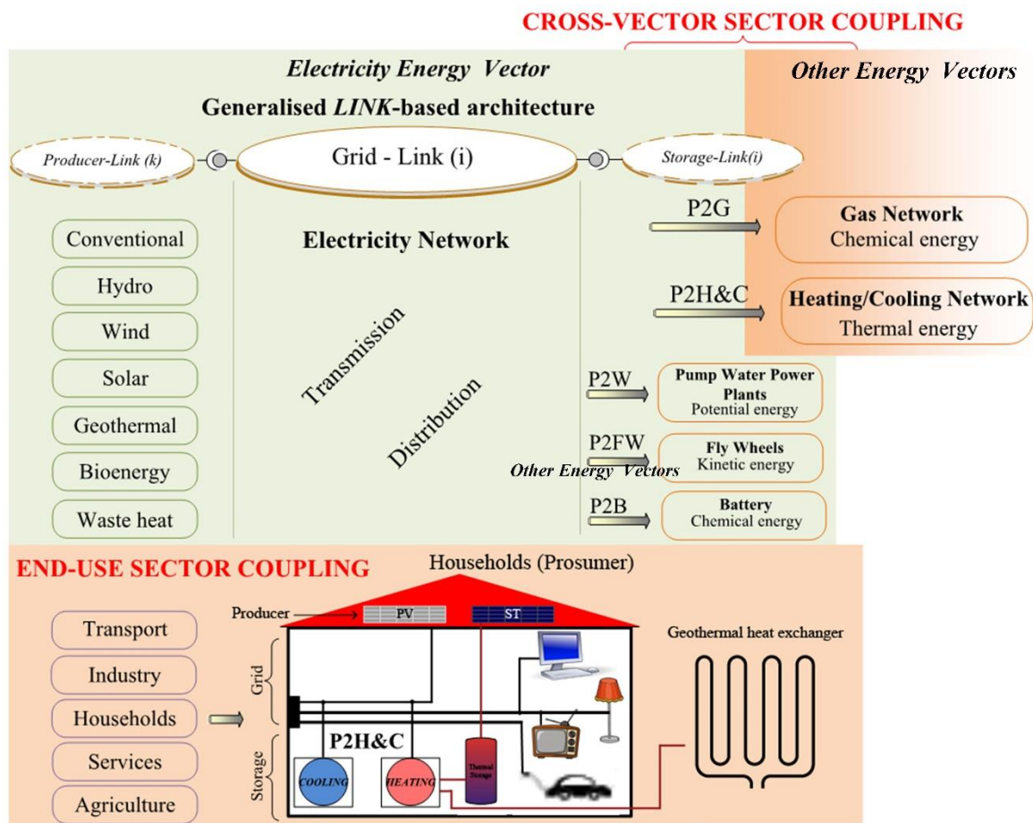
Figure 24. Cross-Vector and End-Use Sector Coupling embedded in the LINK -Solution
