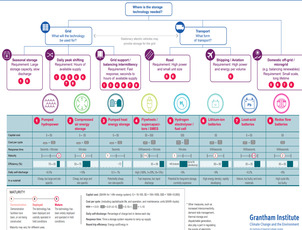
Figure 2.2: Comparative applicability of storage technologies
