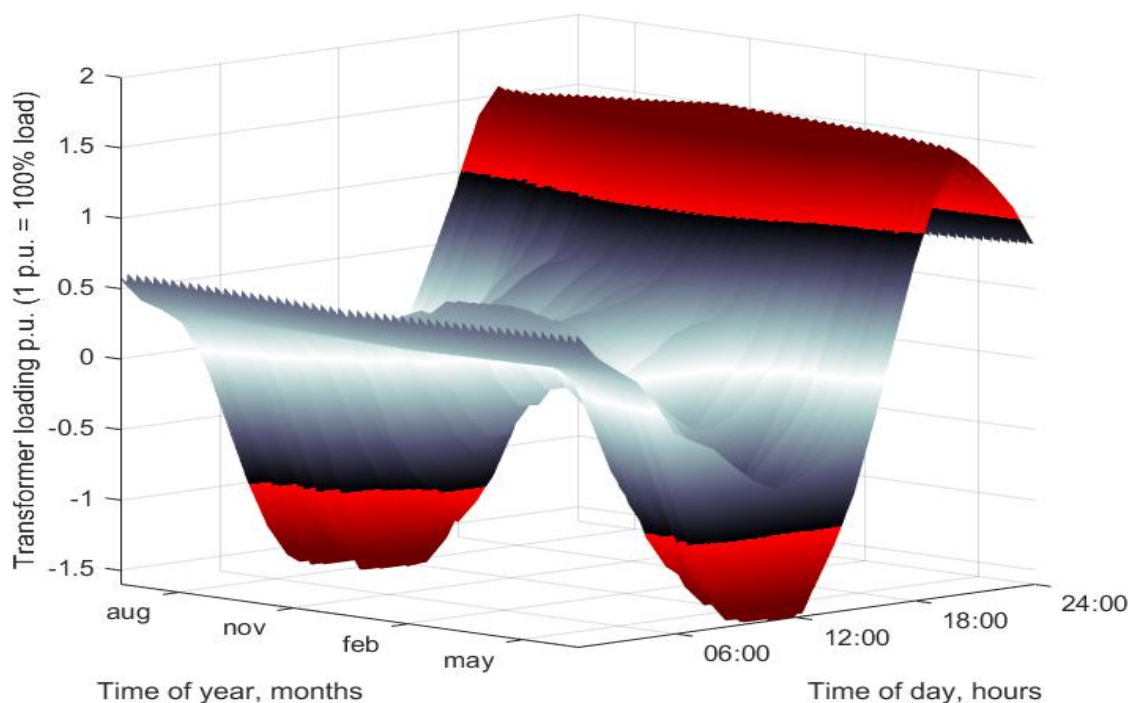
Figure 4.5: Transformer loadings across hours of the day throughout the full year
