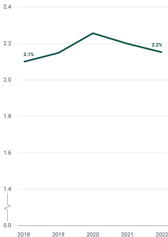
Figure 7.3 Environmental protection expenditure and share of environmental protection expenditure in gross domestic product, EU
