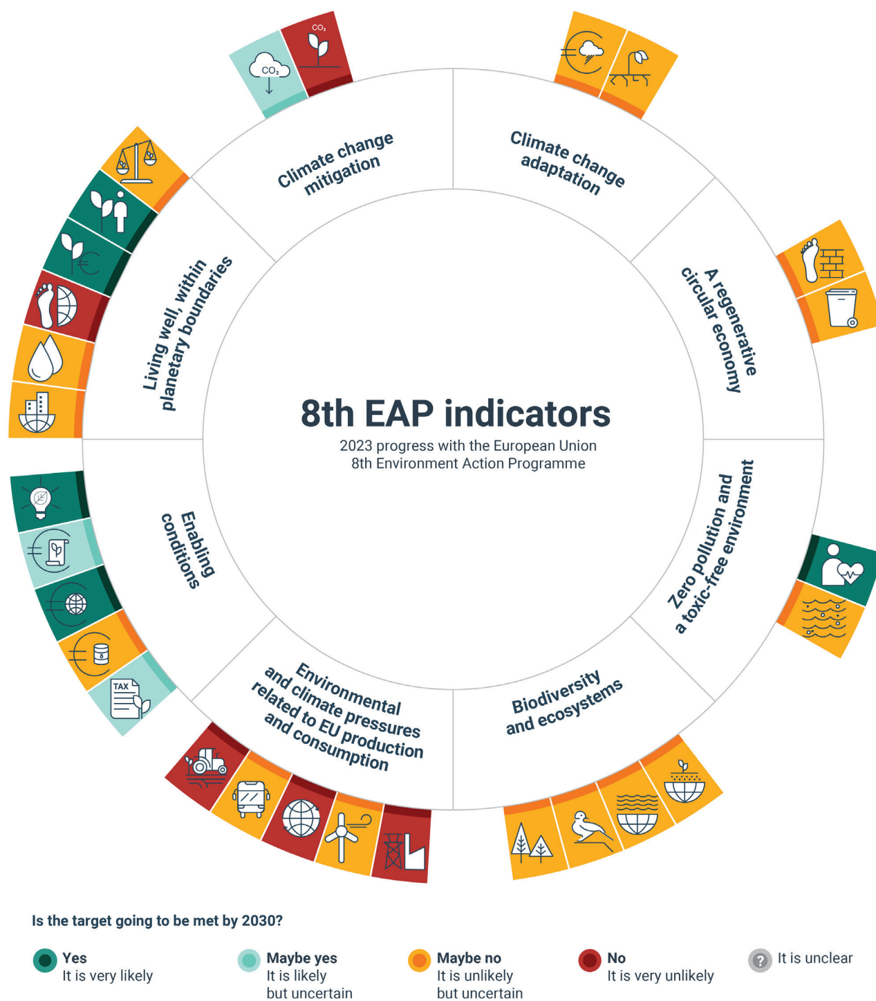
Figure ES.1 8th Environment Action Programme scoreboard, 2023
