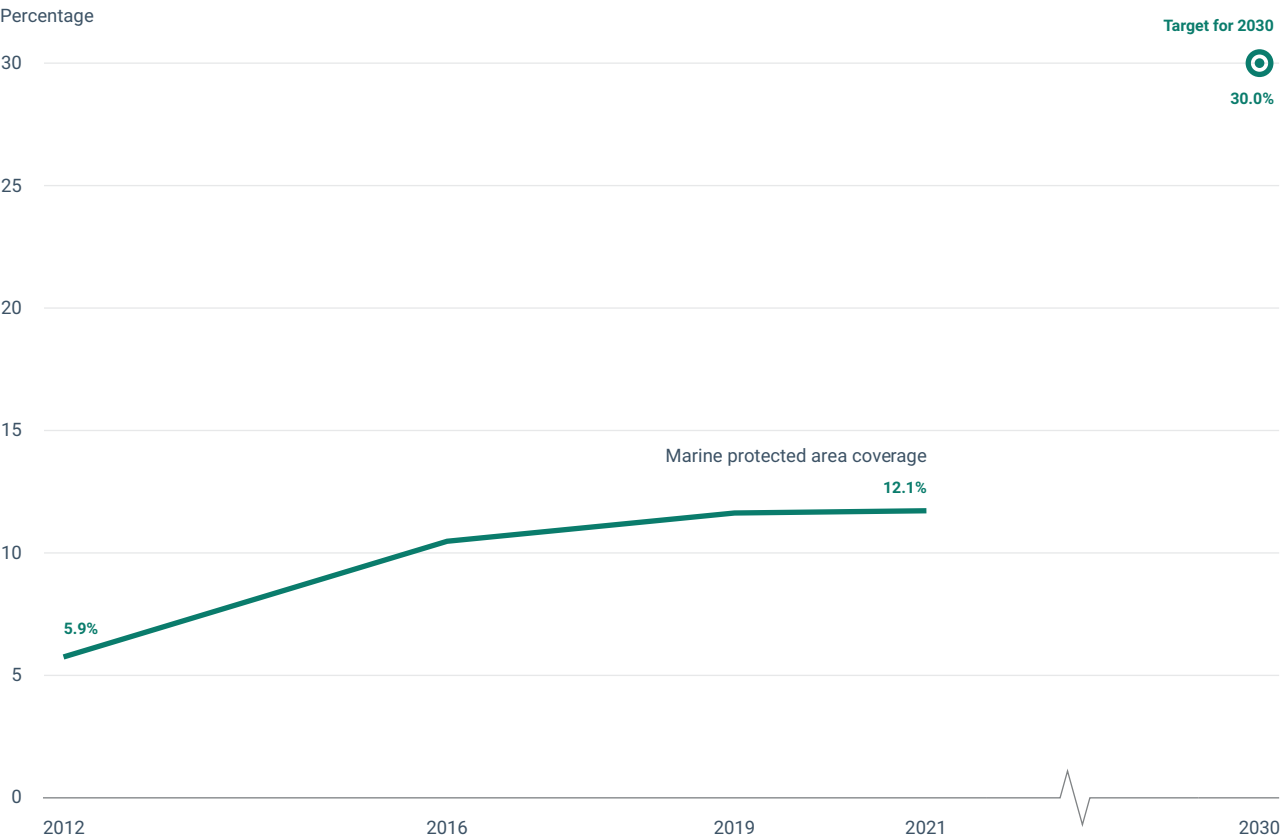
Figure 5.2 Marine protected area coverage, EU
