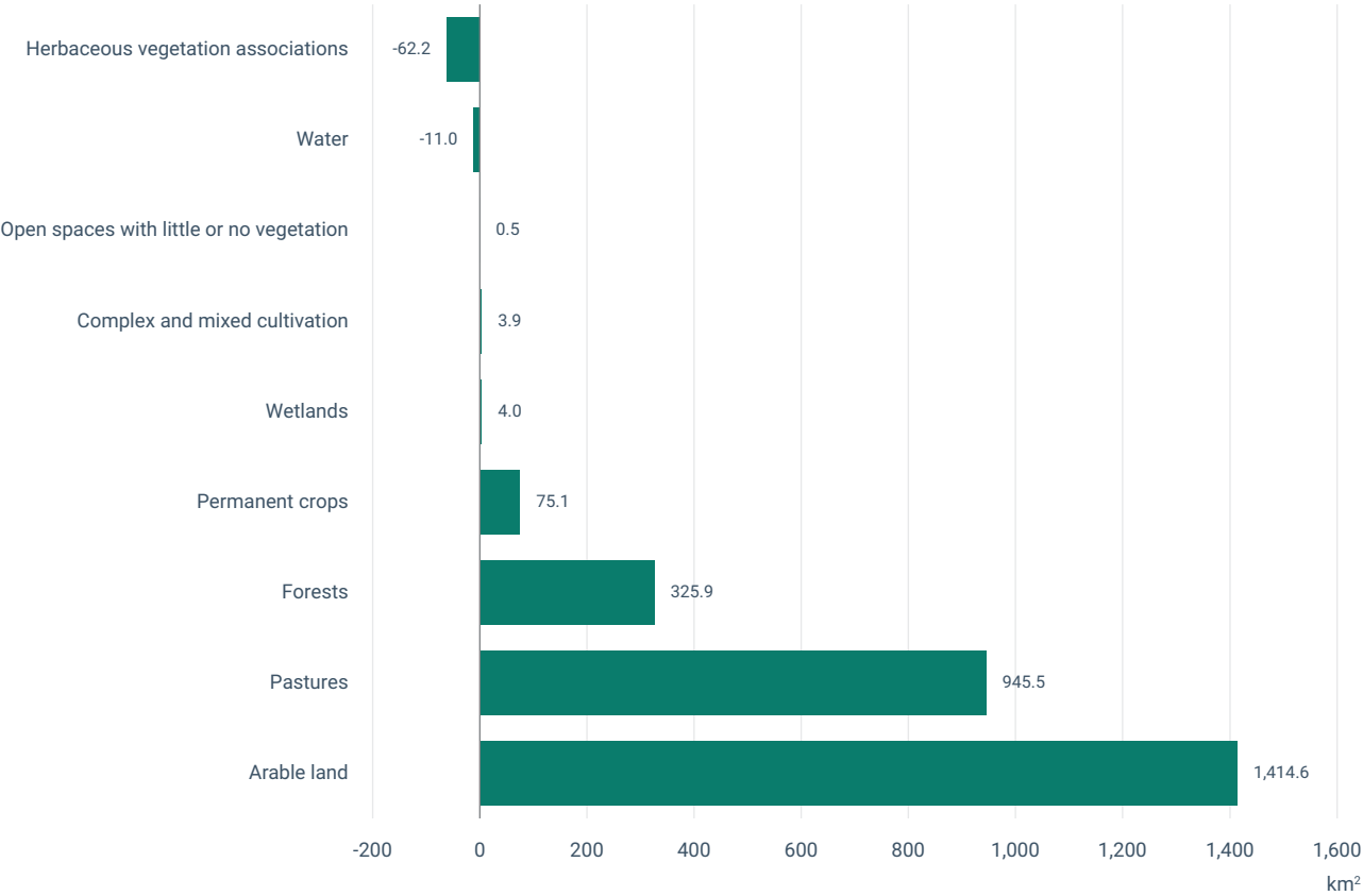
Figure 8.1 Net land take in cities and commuting zones, EU
