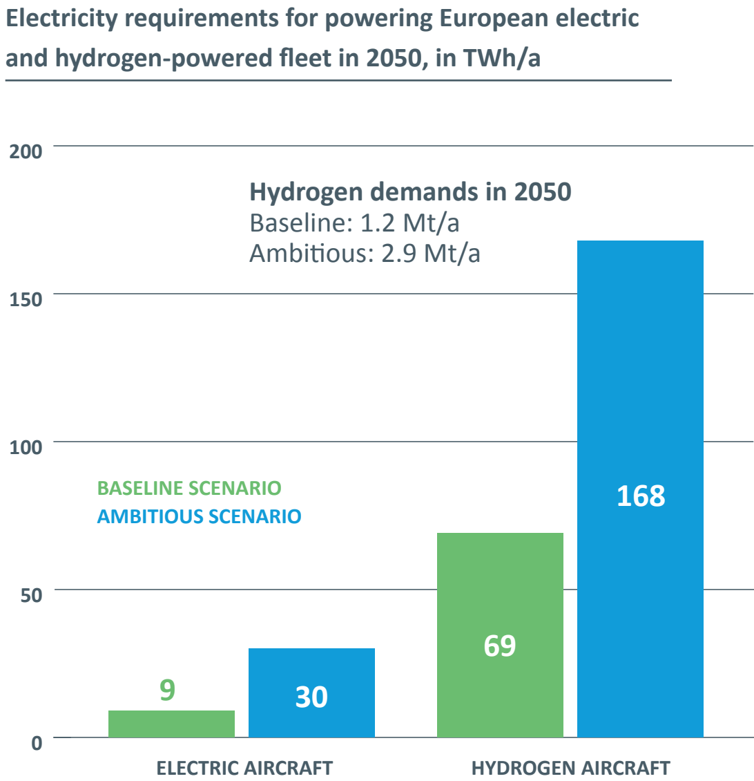
FIGURE 5 Electricity requirements for electric (incl. hybrid) and hydrogen aircraft in 2050 10 .
