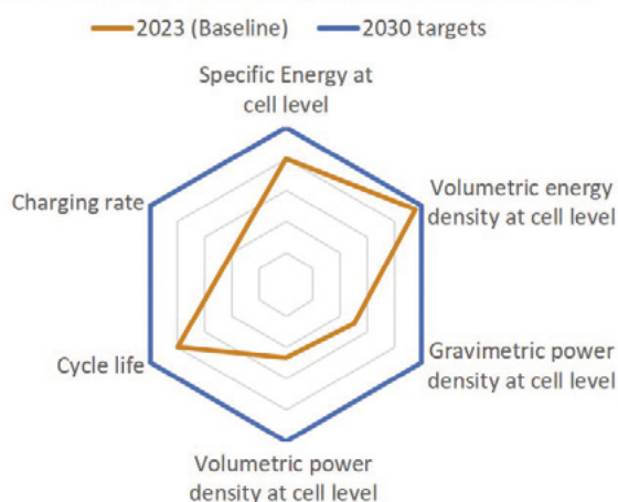
Liquid electrolyte Lithium-ion (Generation 3, Design-to-cost)
