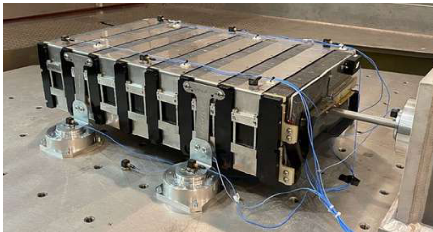
Multi-physical testing of fuel cells
